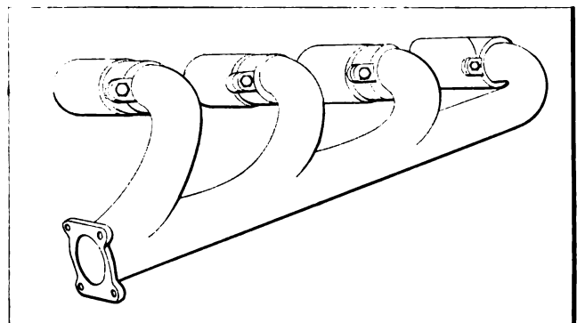
Fig. 13—Manifold so contrived to assure equal distances for all cylinder-ports from depression chamber in carbureter.
